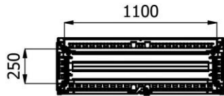
N-N ( 1 :25 )
