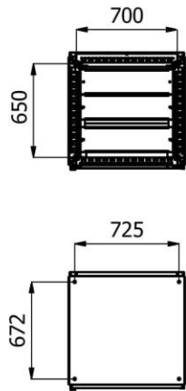
R-R ( 1 :30 )
