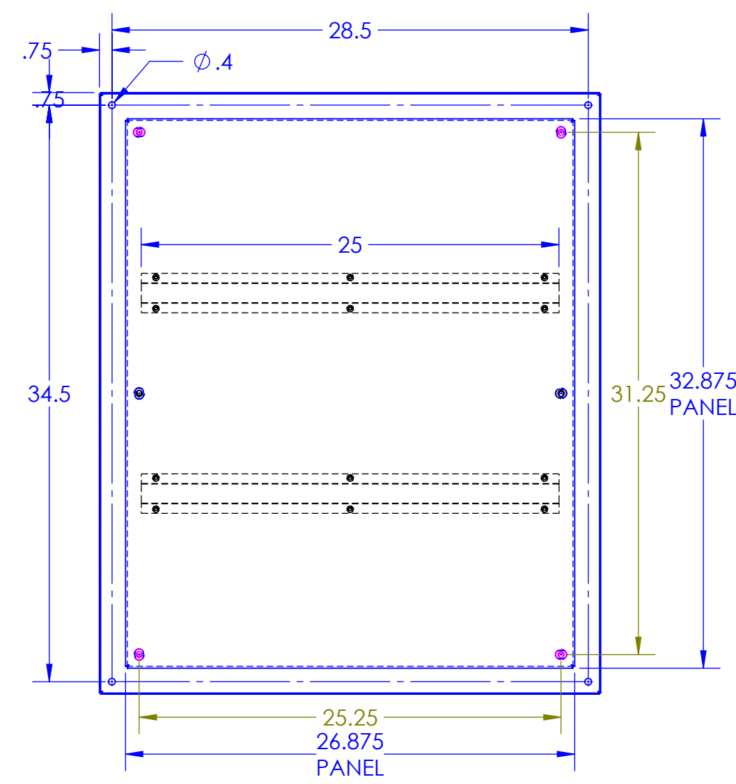
SECTION C-C
