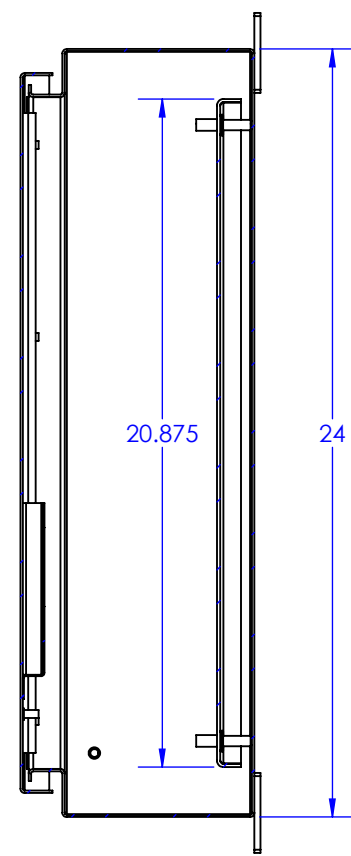
SECTION C-C
