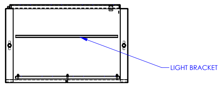
SECTION F-F
