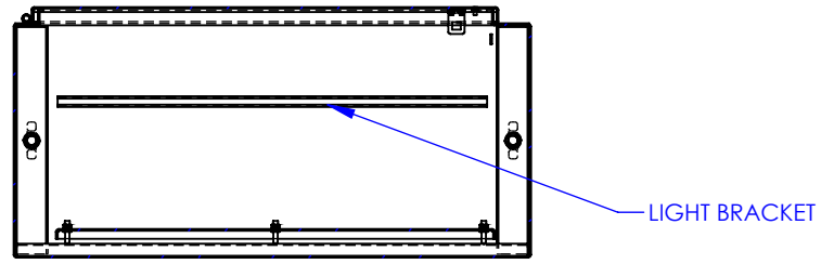
SECTION F-F
