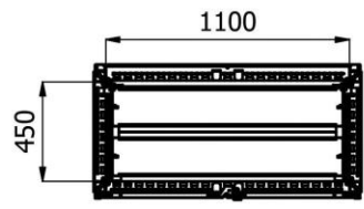
N-N ( 1 :25 )
