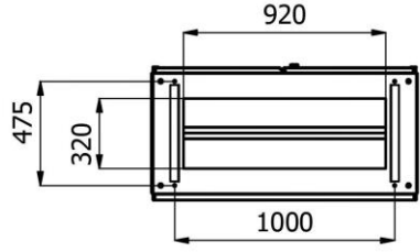
M-M ( 1 :25 )
