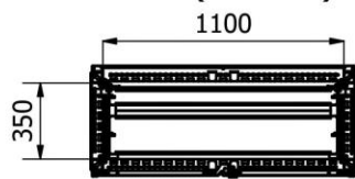
N-N ( 1 :25 )
