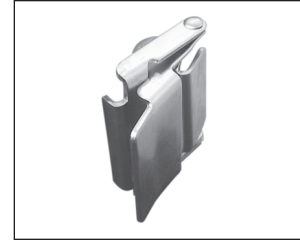
IB SERIES QUICK RELEASE CLAMP Replaces standard clamp (1 per package) JH-40155 – Stainless Steel JH-40165 – Plated Steel
